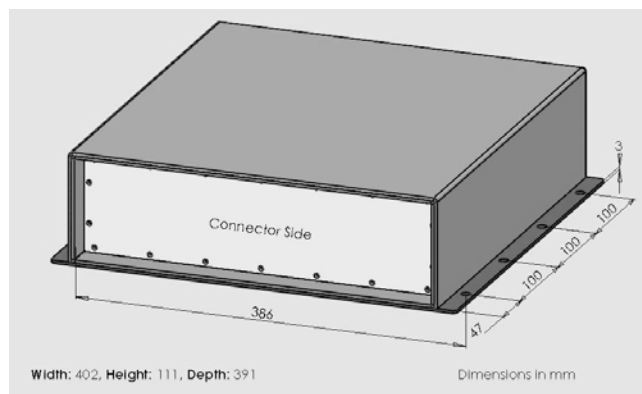
Dimensions of large Outdoor Housing
