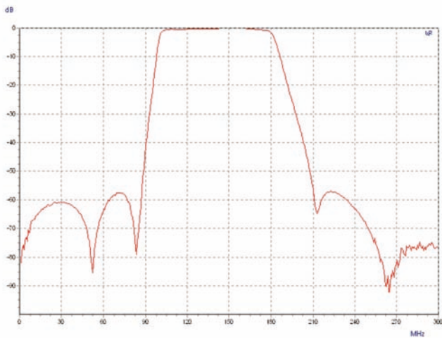
Typical Amplitude-Frequency Response of Response of one 140 MHz Bandpass Filter with 75 MHz 110 MHz Bandwidth.
