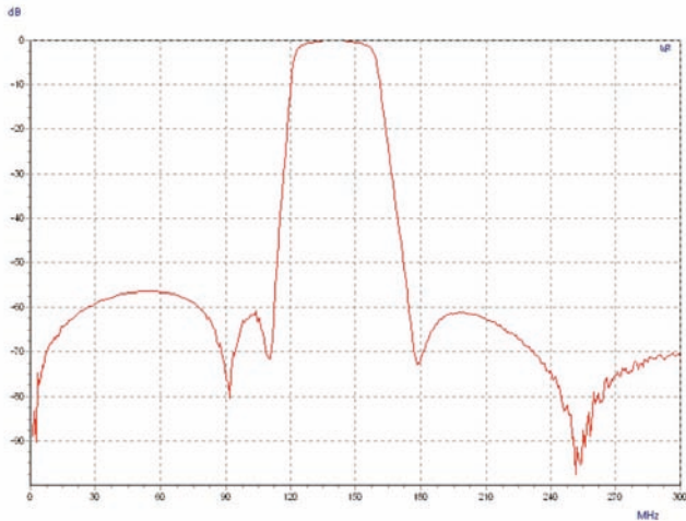
Typical Amplitude-Frequency Response of Response of one 140 MHz Bandpass Filter with 34 MHz 54 MHz Bandwidth.
