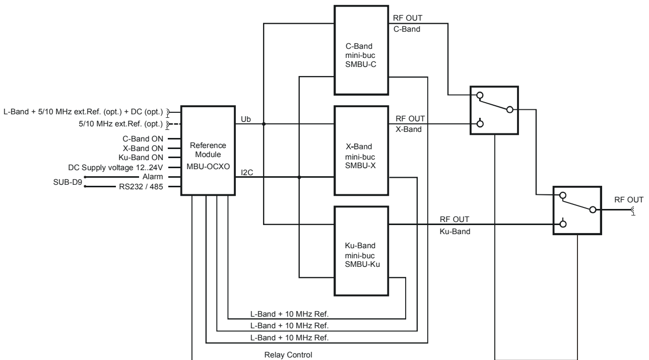
Block diagram of Triple band configuration with reference module
