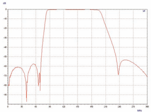
Typical Amplitude-Frequency one 140 MHz Bandpass Filter with Bandwidth.
