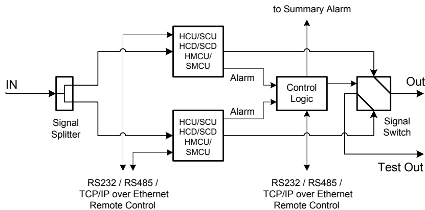
1:1 Redundancy with Signal Splitter
